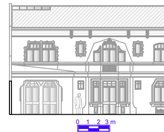
Elevation 03
